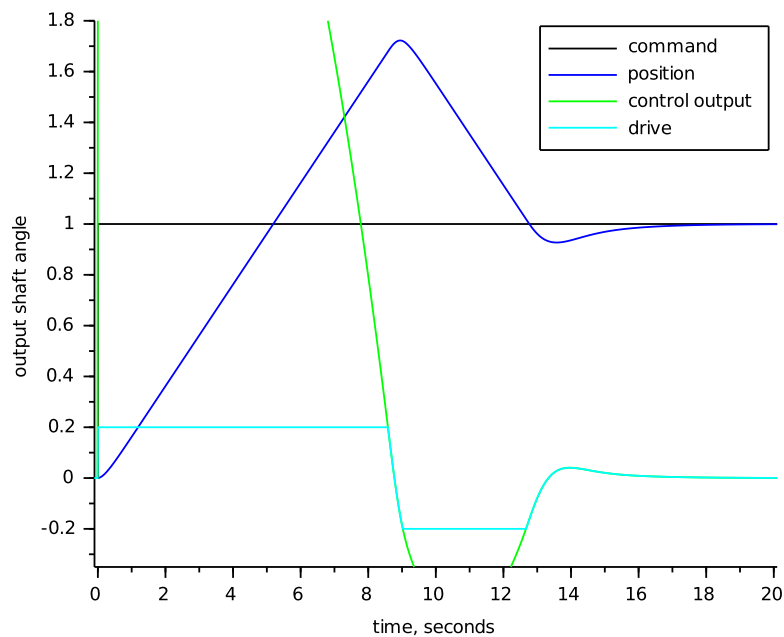
Figure 16: Motor with PI control and windup.
