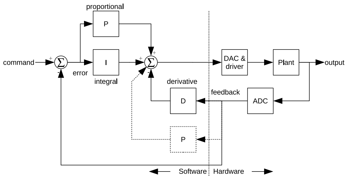
Figure 2: Block diagram of PID controller.
