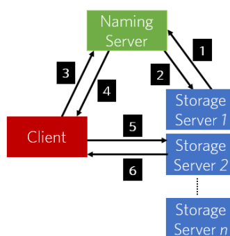
Figure 1: Architecture of FileStack
